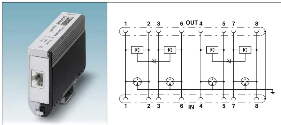
Fig. 98: DT-LAN-Cat.6+ - SPD for information technology
